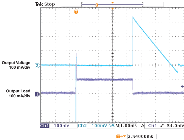
LOAD TRANSIENT RESPONSE VS TIME ( V_{OUT} = 5 V, C_L = 1 \mu F)
