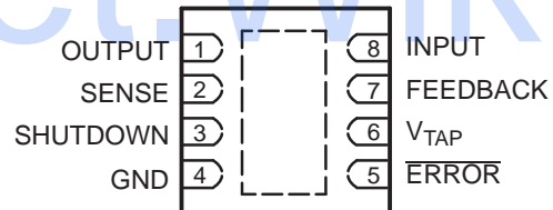
LP2951 . . . DRJ (QFN) PACKAGE (TOP VIEW)
