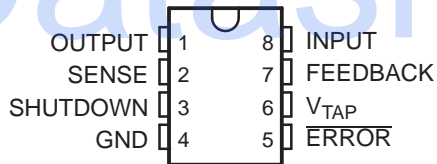
LP2951 . . . D (SOIC) OR DGK (MSOP) PACKAGE (TOP VIEW)
