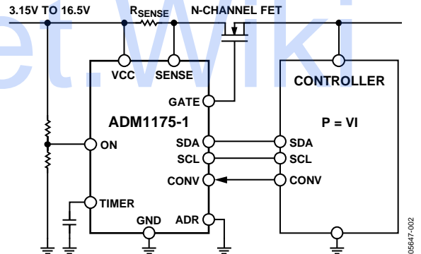
Figure 2. Applications Diagram
