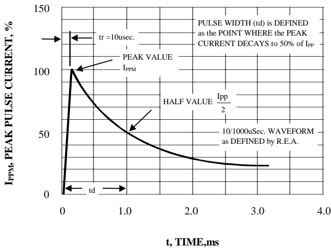
FIG. 3 - PULSE WAVEFORM
